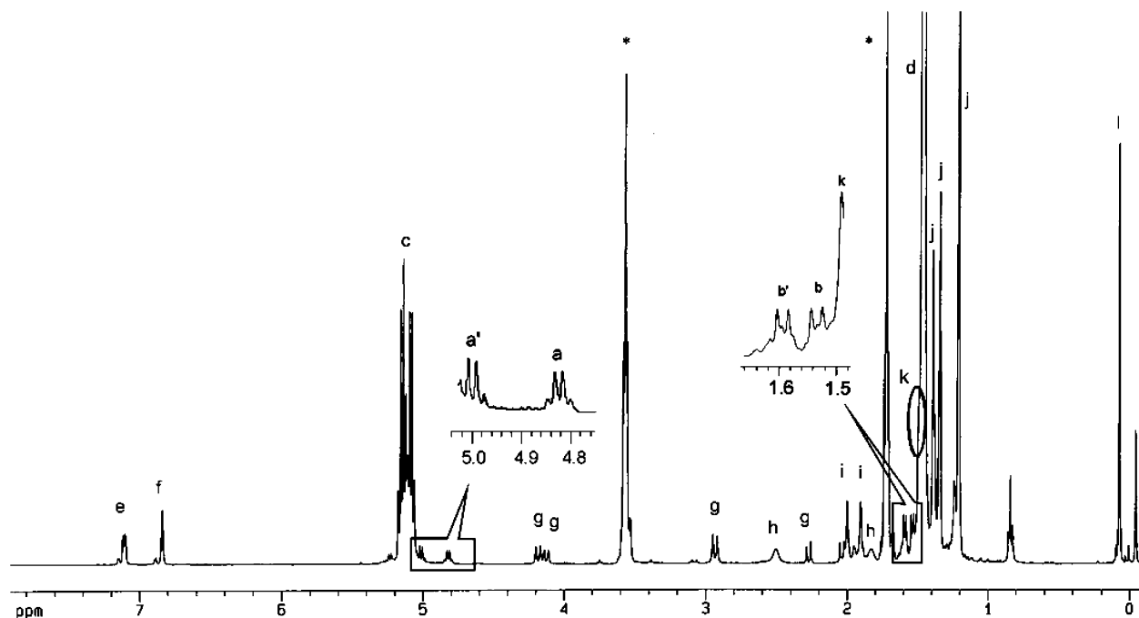
Figure 4. ^1\text{H} NMR spectrum (400 MHz) of the active species of rac -lactide oligomer initiated by complex 1 ( ^*\text{C}_4\text{D}_8\text{O} , [\text{LA}]_0:[\text{Y}] = 15:1 , 25^\circ\text{C} ).
