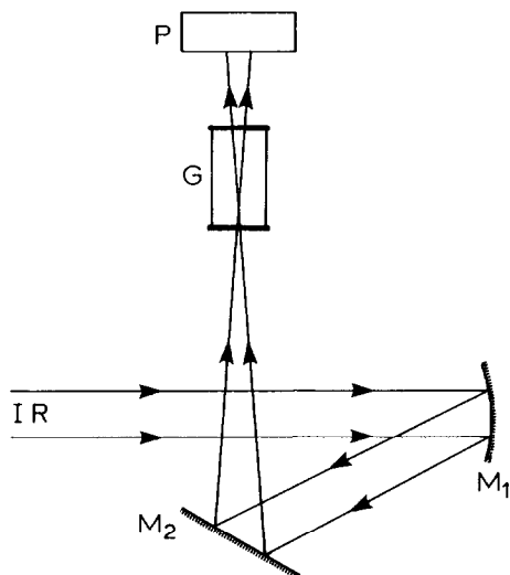
Fig. 1. Optical arrangement for small scale reactions. The IR laser beam, \sim 0.5 cm diameter, is focussed by a concave mirror, M_1 , and plane mirror, M_2 , onto the gas cell, G . The focal length of M_1 is not critical (10–30 cm) but shorter focal lengths tend to crack the windows less frequently. It is convenient to have a power meter, P , to check the laser output.
