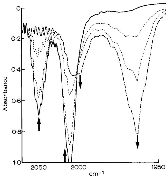
Fig. 2. ^{13}\text{CO} enrichment of \text{Os}(\text{CO})_5 . IR spectra taken before (—), during (-----) and after (— · — · —) 4 min IR laser irradiation (500 mW, P(2O) \text{CO}_2 laser line, 944.2 \text{ cm}^{-1} ), using an arrangement similar to Fig. 1. The laser pyrolysis was stopped while each spectrum was run. Note the change in wave-number scale in the spectrum at 2000 \text{ cm}^{-1} .
