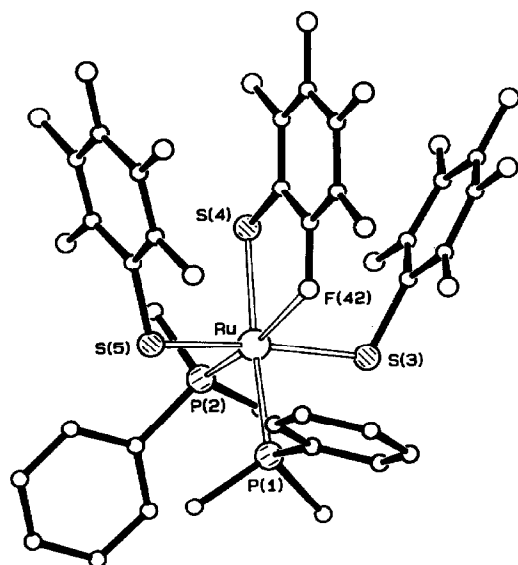
Fig. 2. A molecule of [\text{Ru}\{\text{SC}_6\text{F}_4(\text{F}-2)\}(\text{SC}_6\text{F}_5)_2(\text{PMe}_2\text{Ph})_2] ( B ).
