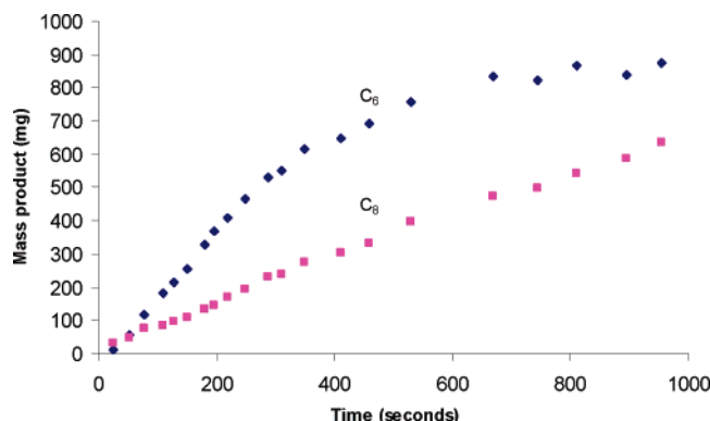
Figure 6. Mass of C_6 and C_8 formed as a function of time for catalysis with 3 equiv of Al(OC_6F_5)_3 ( 2 ). Conditions: 10 \mu mol of CrCl_3(thf)_3 , 12 \mu mol of II , 30 AlEt_3 , 45 ^\circ C , 40 bar.
