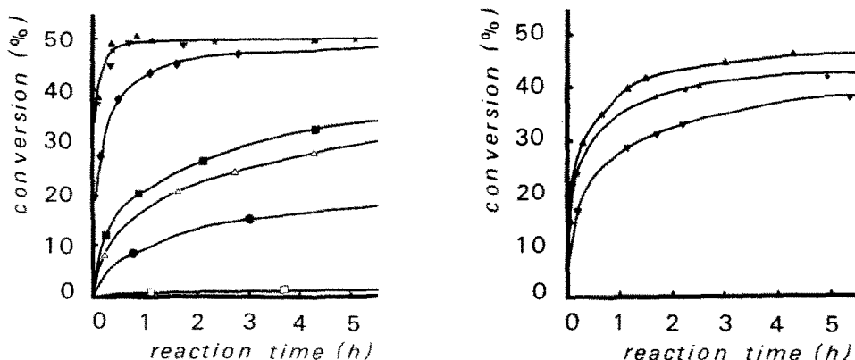
Fig. 1. Effect of different cocatalysts on the metathesis of methyl oleate in the presence of \text{Re}_2\text{O}_7/\text{Al}_2\text{O}_3 (126 \mu\text{l}/100 mg \text{Re}_2\text{O}_7/\text{Al}_2\text{O}_3 ) \star \text{Sn}(\text{CH}_3)_4 , \blacktriangle \text{Sn}(\text{C}_2\text{H}_5)_4 , \blacktriangledown \text{Sn}(\text{C}_4\text{H}_9)_4 , \blacklozenge \text{Sn}(\text{C}_8\text{H}_{17})_4 , \blacksquare (\text{CH}_3)_3\text{Al}_2\text{Cl}_3 , \triangle \text{Sn}(\text{i-C}_3\text{H}_7)_4 , \bullet \text{Sn}(\text{C}_6\text{H}_{11})_4 , \square \text{Li}(\text{C}_4\text{H}_9)_4 .
