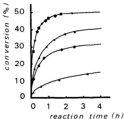
Fig. 3. Effect of the \text{Re}_2\text{O}_7 content of the \text{Re}_2\text{O}_7/\text{Al}_2\text{O}_3\text{-Sn}(\text{CH}_3)_4 catalyst on the metathesis of methyl oleate. \blacktriangle 6 mass% \text{Re}_2\text{O}_7 , \blacksquare 9 mass% \text{Re}_2\text{O}_7 , \blacklozenge 12 mass% \text{Re}_2\text{O}_7 , \star 15 mass% \text{Re}_2\text{O}_7 , \bullet 18 mass% \text{Re}_2\text{O}_7 .
