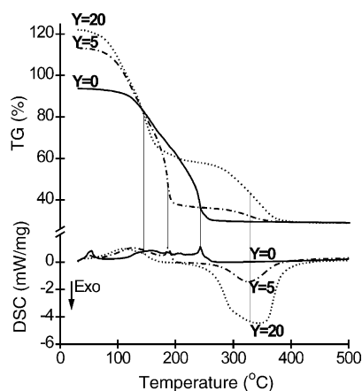
Fig. 3. TG and DSC curves of Mn–Co nitrate supported on varying amounts of carbon, measured in air ( 5 \text{ K min}^{-1} ).
