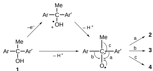
Scheme 2 \beta -Fragmentation of a possible alkoxyl radical intermediate (Ar = phenyl and Ar' = p -carboxyphenyl)
