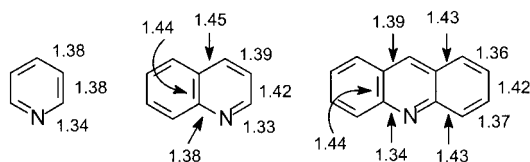
Scheme 3. Bond lengths [Å] in pyridine, quinoline, and acridine (averages of different X-ray data reported in the literature for alkyl derivatives).
