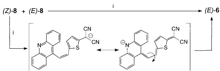
Scheme 6. Preparation of the E diastereoisomer of the acridine-based sodium salt 6 from both the E and the Z forms of the precursor bromo derivative 8 : i) CH 2 (CN) 2 , NaH, DME, [Pd(PPh 3 ) 4 ], RT.
