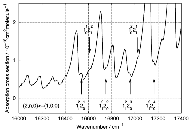
Figure 5. Newly observed vibrational bands in the visible absorption spectrum of OBrO. The arrows below the spectrum curve mark the bands that belong to the progression (2, \nu'_2, 0)\text{--}(1, 0, 0) . The labels indicate the \nu_1 vibrational transitions by 1_n'' and the \nu_2 transitions by 2_n'' . The spectral resolution is 8\text{ cm}^{-1} .
