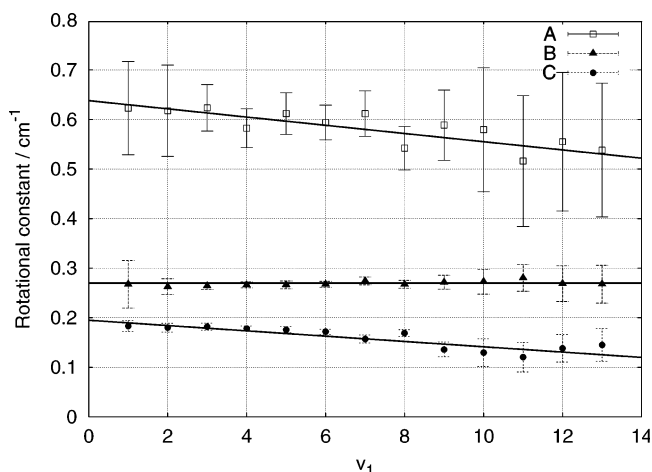
Figure 8. Rotational constants A, B, and C for the electronic state C( 2 A 2 ). The values for different rovibrational bands in the progression (\nu_1, 0, 0) \leftarrow (0, 0, 0) are plotted against the vibrational quantum number \nu_1 . The error bars represent a 2σ uncertainty.
