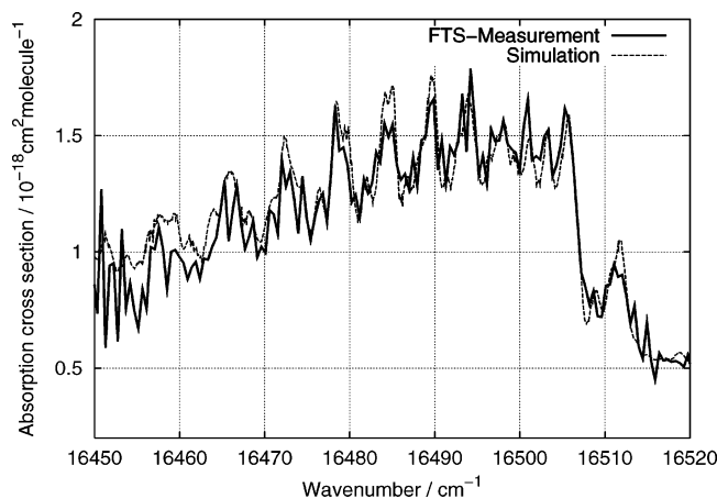
Figure 6. Comparison of experimental and simulated absorption spectrum for the rovibrational band (1,0,0)–(0,0,0). The spectral resolution was 0.8\text{ cm}^{-1} (fwhm) for the experimental spectrum and 0.15\text{ cm}^{-1} for the synthesized spectrum. For the simulated spectrum, a line width of 0.8\text{ cm}^{-1} (fwhm) was used.
