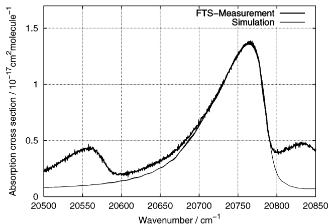
Figure 7. Comparison of experimental and simulated absorption spectrum for the rovibrational band (8,0,0)–(0,0,0). The spectral resolution was 0.8\text{ cm}^{-1} (fwhm) for the experimental spectrum and 0.15\text{ cm}^{-1} for the synthesized spectrum. For the simulated spectrum, a line width of 10\text{ cm}^{-1} (fwhm) was used.
