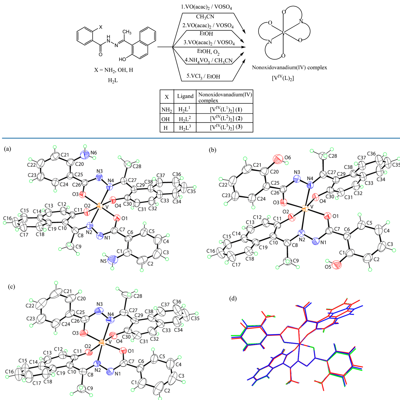
Figure 1. Molecular structures of 1 (a), 2 (b), 3 (c) and overlay diagram of 1 (red image), 2 (green) and 3 (blue) drawn so that the V, O1 and O2 atoms are coincident (d).
