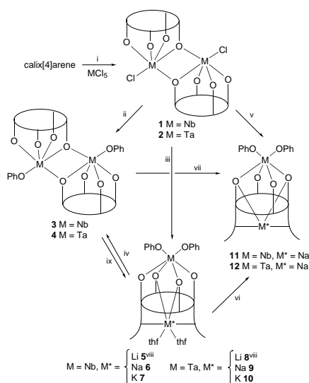
Scheme 1 Reagents and conditions: i, toluene, reflux; ii, 1 equiv. NaOPh, thf, room temp.; iii, excess of M + OPh, thf; iv, 1 equiv. of 1 in thf or 1 equiv. of 2 in C 6 H 6 ; v, 2 equiv. NaOPh, C 6 H 6 , reflux; vi, azeotropic distillation, C 6 H 14 ; vii, excess of NaOPh, C 6 H 6 ; viii, a single thf is bonded to Li + ; ix, NaOPh, thf, room temp.
