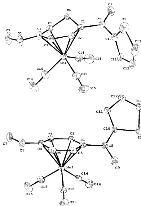
Figure 1. ORTEP representations of complexes 7 and 11 with thermal ellipsoids at the 30% probability level. Selected bond lengths for 7 (Å): C8–C9 1.344(4), C1–C8 1.484(3), C8–C10 1.497(4), C1–C2 1.415(3), C2–C3 1.431(3), C3–C4 1.427(4), C4–C5 1.409(3), C5–C6 1.518(4), C6–C1 1.528(3), Mn–C1 2.285(2), Mn–C2 2.148(2), Mn–C3 2.148(2), Mn–C4 2.215(3), Mn–C5 2.229(2). For 11 : C8–C9 1.342(3), C1–C8 1.499(3), C8–C10 1.470(3), C1–C2 1.431(3), C2–C3 1.406(3), C3–C4 1.423(3), C4–C5 1.408(3), C5–C6 1.420(3), Mn–C1 2.206(2), Mn–C2 2.1713(19), Mn–C3 2.196(2), Mn–C4 2.282(2), Mn–C5 2.212(2), Mn–C6 2.190(2).
