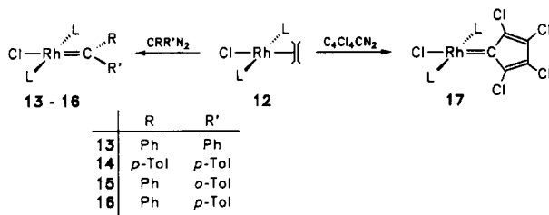
Scheme 6. (L = \text{Sb}i\text{Pr}_3 ).
