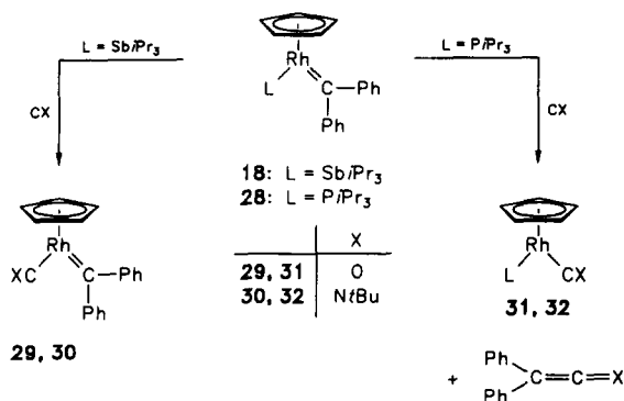
Scheme 9.
