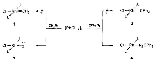
Scheme 2. (L = \text{PiPr}_3 ).
