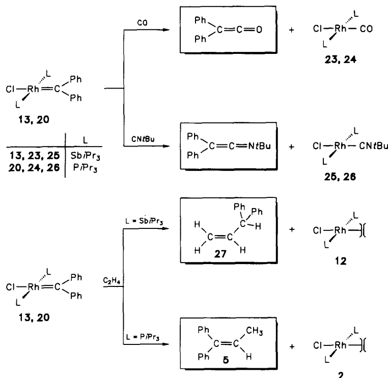
Scheme 8.
