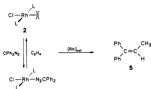
Scheme 3. (L = \text{PiPr}_3 ).
