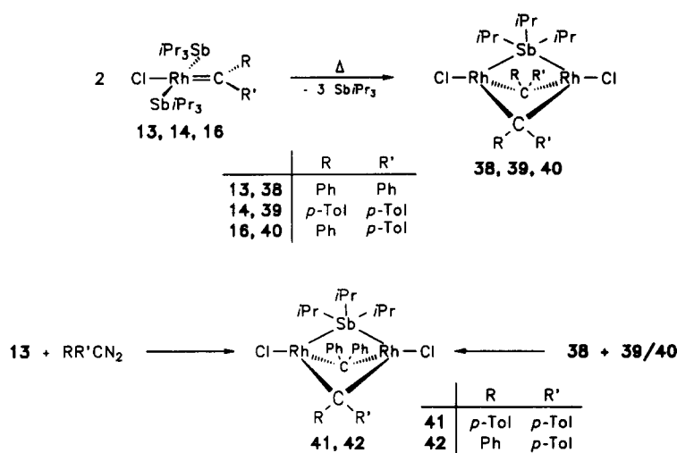
Scheme 11.
