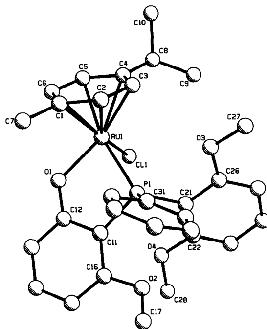
Fig. 2. Molecular structure of (\eta^6\text{-}p\text{-cymene})\text{RuCl}[\text{PPh}\{\text{2,6-(MeO)}_2\text{C}_6\text{H}_3\}\{\text{2-O-6-MeOC}_6\text{H}_3\}] 3b .
