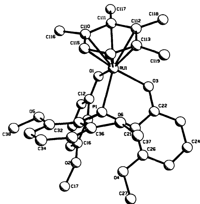
Fig. 1. Molecular structure of [(\eta^6\text{-}1,2,3,4\text{-Me}_4\text{C}_6\text{H}_2)\text{Ru}\{\text{P}[\text{2,6-(MeO)}_2\text{C}_6\text{H}_3]\{\text{2-O-6-MeOC}_6\text{H}_3\}_2\}] 2a .
