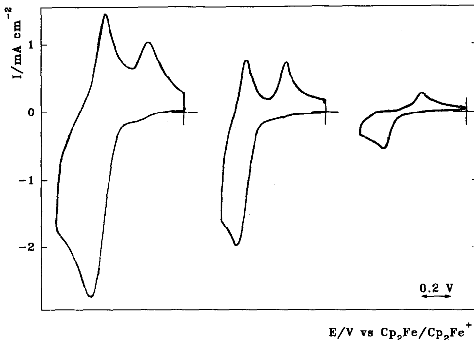
Fig. 4. Cyclic voltammograms for the complex IIa (7 mM) in THF/ \text{Bu}_4\text{NBF}_4 (0.2 M). Vitreous carbon disc electrode. Potential scan rates are 36, 225 and 400 \text{mV s}^{-1} . The initial potential for each scan was -0.60 V.
