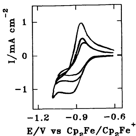
Fig. 6. Cyclic voltammograms for the complex IIa (19 mM) in THF/Bu 4 NBF 4 (0.2 M) where the Bu 4 NBF 4 has been poorly dried and hence the medium contains some water. Vitreous carbon disc electrode. Potential scan rates are 75, 100 and 600 mV s -1 . The negative potential limit is restricted so that CpTiCl 2 (OH) but not CpTiCl 2 (OR) is reduced.
