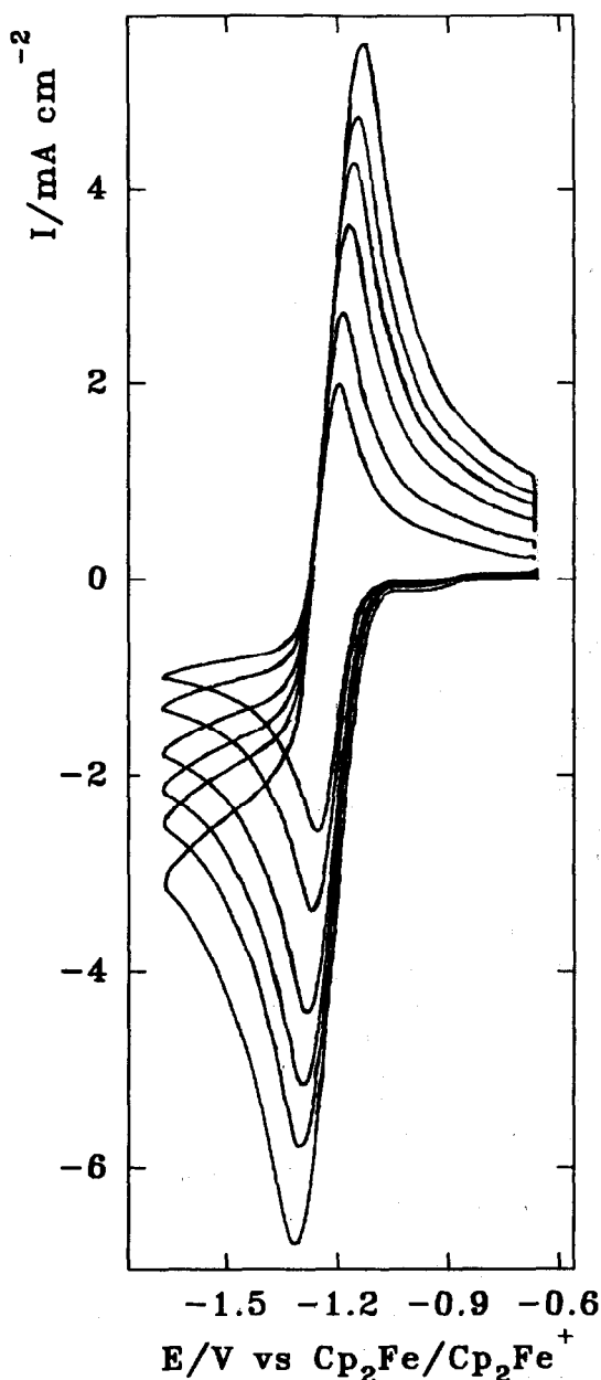
Fig. 2. Cyclic voltammograms for the complex Id (11 mM) in THF/Bu 4 NBF 4 (0.2 M). Vitreous carbon disc electrode. Potential scan rates are 50, 100, 200, 300, 400 and 600 mV s -1 .
