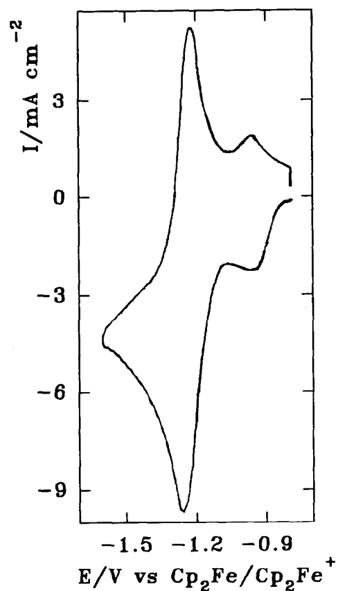
Fig. 5. Cyclic voltammograms for the complex Id (21 mM) in THF/ \text{Bu}_4\text{NBF}_4 (0.2 M) where the \text{Bu}_4\text{NBF}_4 has been poorly dried and hence the medium contains some water. Vitreous carbon disc electrode. Potential scan rate is 400 \text{ mV s}^{-1} .
