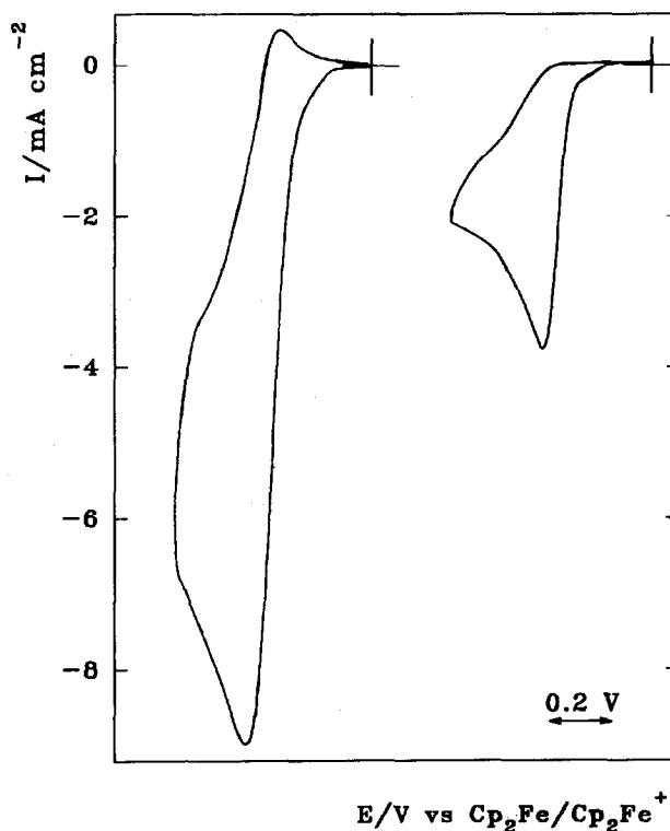
Fig. 3. Cyclic voltammograms for the complex Ie ( 14\ \text{mM} ) in \text{THF}/\text{Bu}_4\text{NBF}_4 ( 0.2\ \text{M} ). Vitreous carbon disc electrode. Potential scan rates are 100 and 800\ \text{mV}\ \text{s}^{-1} and the scans were each commenced from -0.66\ \text{V} .
