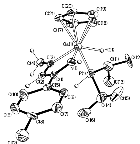
Figure 2. Molecular diagram of the cation of [\text{OsH}(\eta^5\text{-C}_5\text{H}_5)\{\text{NH}=\text{C}(p\text{-C}_6\text{H}_4\text{Cl})\text{CH}=\text{C}(\text{CH}_3)\}(\text{PH}^i\text{Pr}_2)]\text{BF}_4 ( 10 ).
