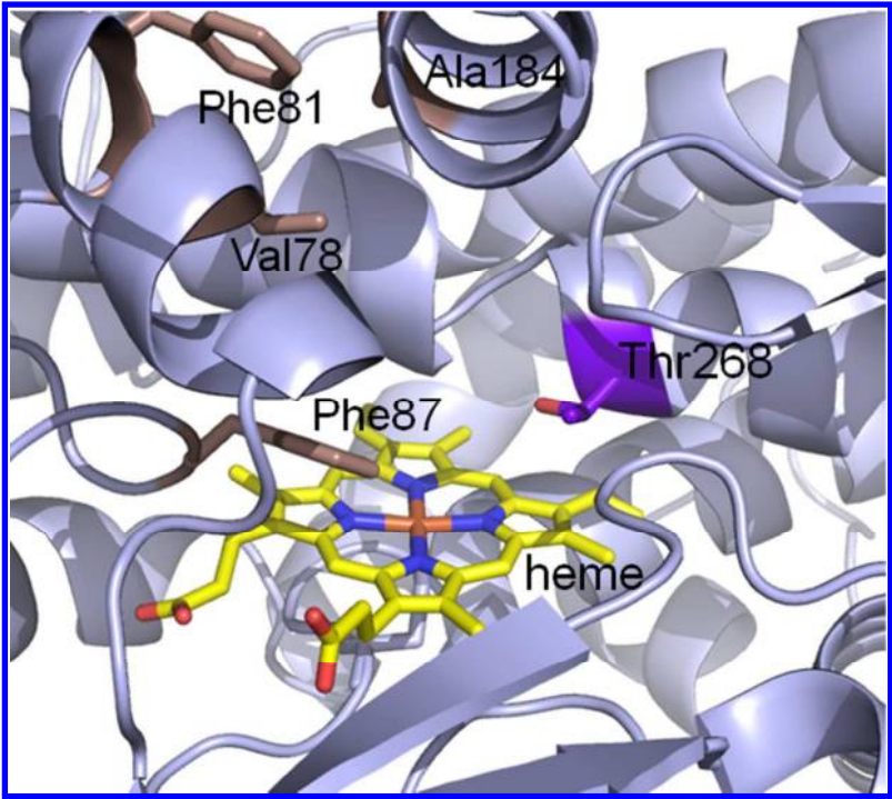
Figure 2. Close-up view of active site cavity in the substrate-bound structure of P450 BM3 (pdb 1FAG 48 ). The heme cofactor and Thr268 residue are highlighted in yellow and purple, respectively. Active site positions that are mutated in the P450 variants tested in this study are also labeled (brown, see Table S1). The enzyme-bound substrate (palmitate) and part of the protein structure is not shown for clarity.
