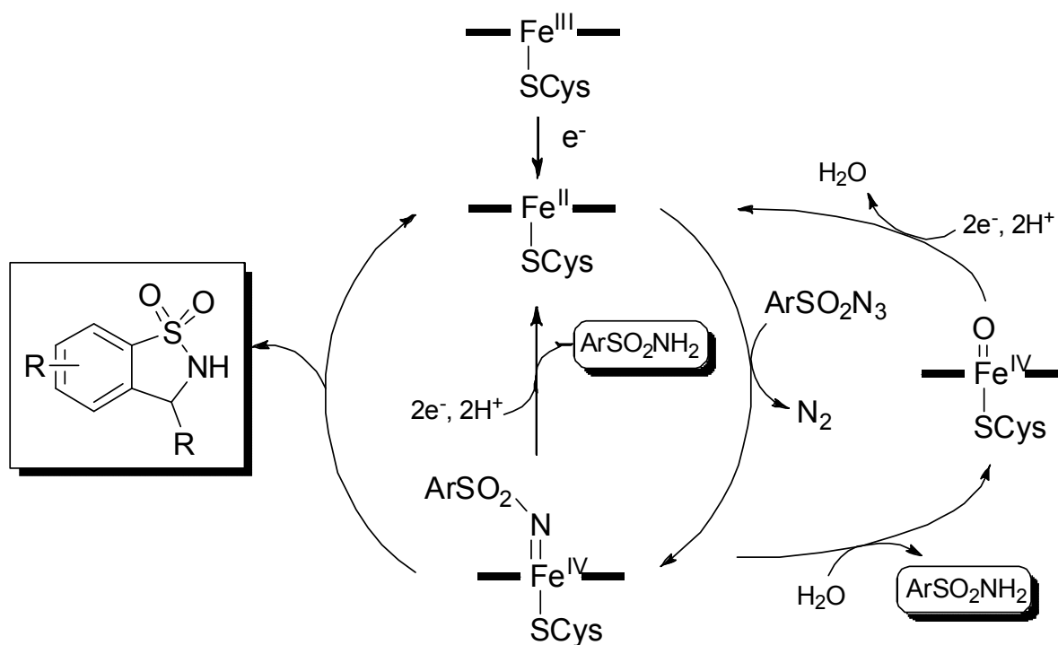
Scheme 1. Proposed mechanism for the formation of the benzosultam and benzosulfonamide products in the P450-catalyzed reactions.
