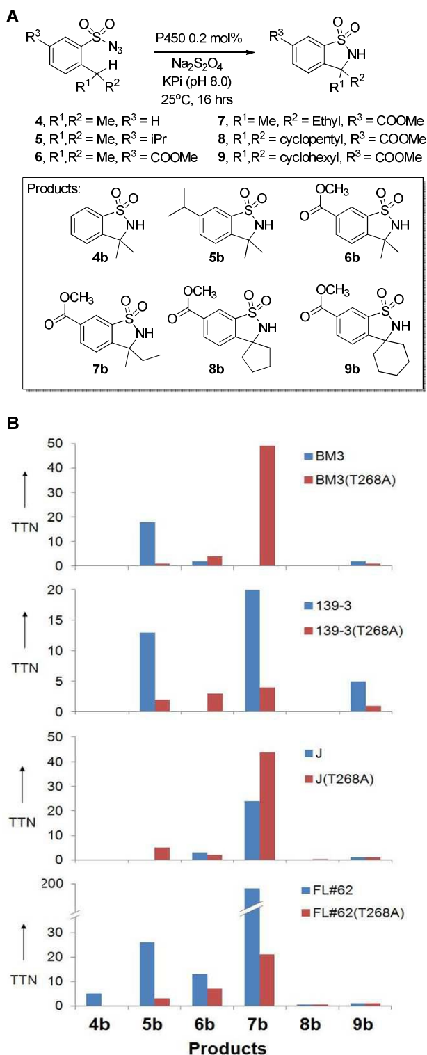
Figure 1. Substrate scope of P450 C—H amination catalysts. A) Tested substrates and corresponding benzosultam products. B) Measured TTNs for the different P450 variants (see also Table S2 ).
