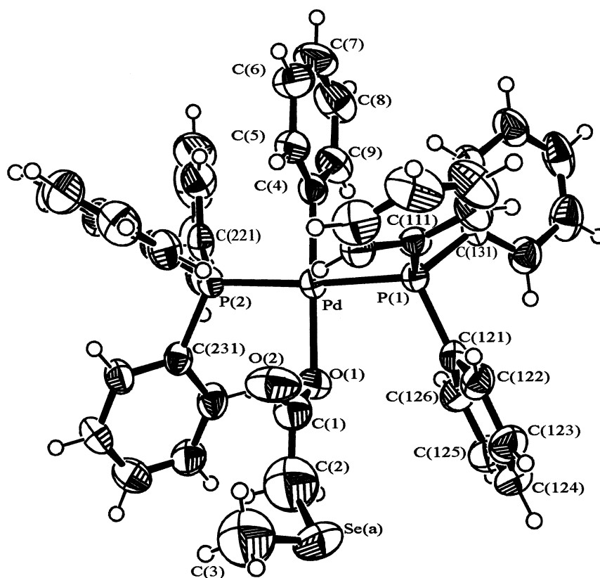
Fig. 5. ORTEP plot of the molecular structure of complex 1h (one of two disordered configurations), showing the numbering scheme.
