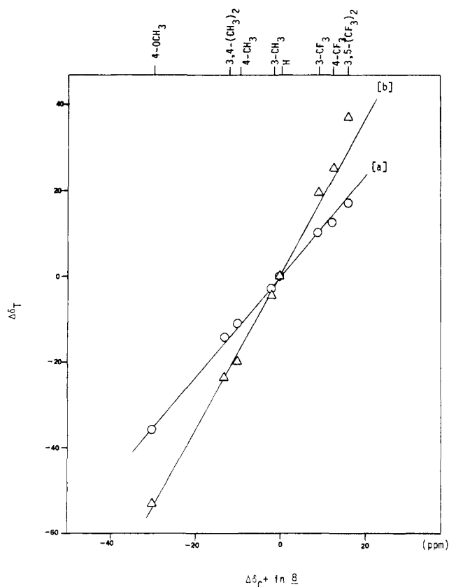
Figure 3. A plot of the differential sum of C_\alpha and C_\gamma chemical shifts of 1-aryl-3-methylbut-2-enyl cations ( 2 ) [a, O] and 2-arylpent-3-yn-2-yl cations ( 3 ) [b, Δ] vs. differential carbocationic center chemical shifts of 1-aryl-1-cyclopentyl cations ( 8 ).
