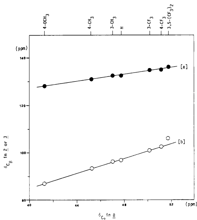
Figure 2. A plot of \delta_{\text{C}\beta} 's in 1-aryl-3-methylbut-2-enyl cations ( 2 ) [a] and 2-aryl-3-pent-2-enyl cations ( 3 ) [b] vs. \delta_{\text{C}_2} in 1-aryl-1-cyclopentyl cations ( 8 ).
