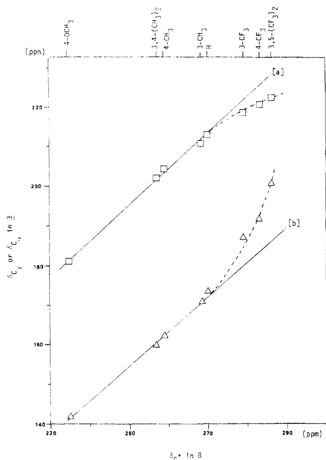
Figure 5. A plot of C_\alpha [a] and C_\gamma [b] chemical shifts of 2-arylpent-3-yn-2-yl cations ( 3 ) vs. carbocationic center chemical shifts of 1-aryl-1-cyclopentyl cations ( 8 ).
