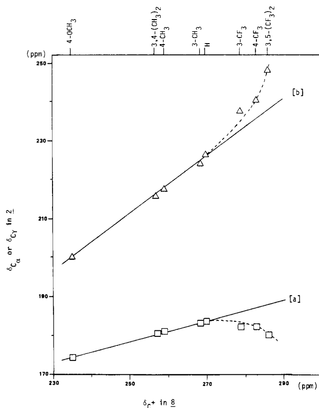
Figure 1. A plot of \text{C}_\alpha [a] and \text{C}_\gamma [b] chemical shifts of 1-aryl-3-methylbut-2-enyl cations ( 2 ) vs. carbocationic center chemical shifts of 1-aryl-1-cyclopentyl cations ( 8 ).
