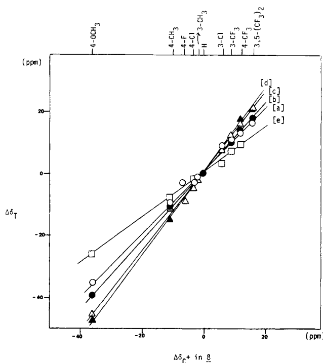
Figure 6. A plot of the differential sum of ortho, para, and carbocationic center chemical shifts of diarylethyl cations ( 14 [a, ○], 15 [b, ●], 16 [c, ▲], 17 [d, △]) and 9-methylantracenium cations ( 19 ) [e, □] vs. the differential carbocationic center chemical shifts of 1-aryl-1-cyclopentyl cations ( 8 ).
