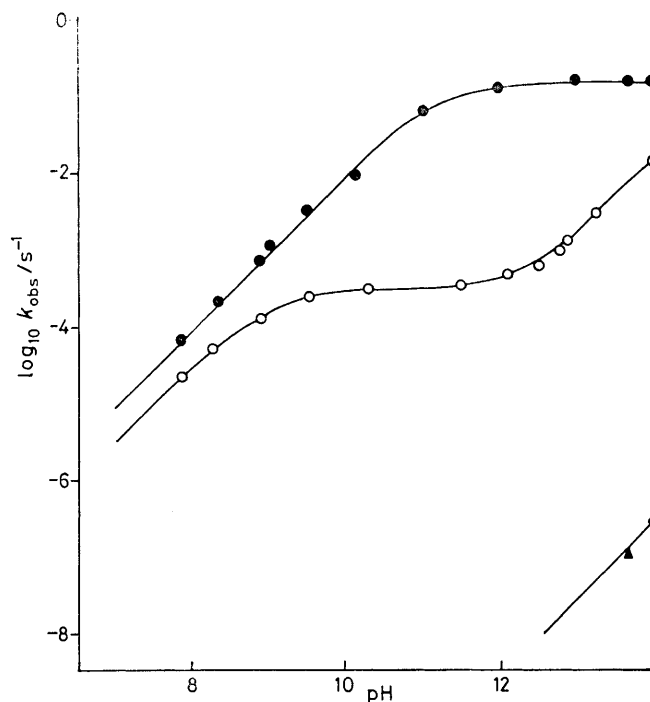
FIGURE. Dependence on pH of the hydrolysis of 4-nitrophenyl methylsulphonylmethanesulphonate (open circles) and its \alpha -methyl- (closed circles) and \alpha\alpha -dimethyl- (closed triangles) substituted analogues in water at 25 °C.
