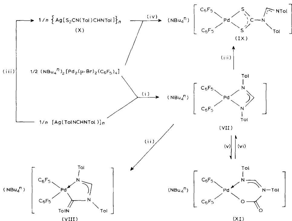
Scheme 1. (i) \text{CH}_2\text{Cl}_2 , 1 day; (ii) stoichiometric amount of \text{CNTol} , \text{CH}_2\text{Cl}_2 , 10 min; (iii) \text{CS}_2 in \text{CH}_2\text{Cl}_2 , 1 h; (iv) \text{CH}_2\text{Cl}_2 , 15 h; (v) \text{CH}_2\text{Cl}_2 , bubbling \text{CO}_2 ; (vi) spontaneously or on bubbling of \text{N}_2 .
