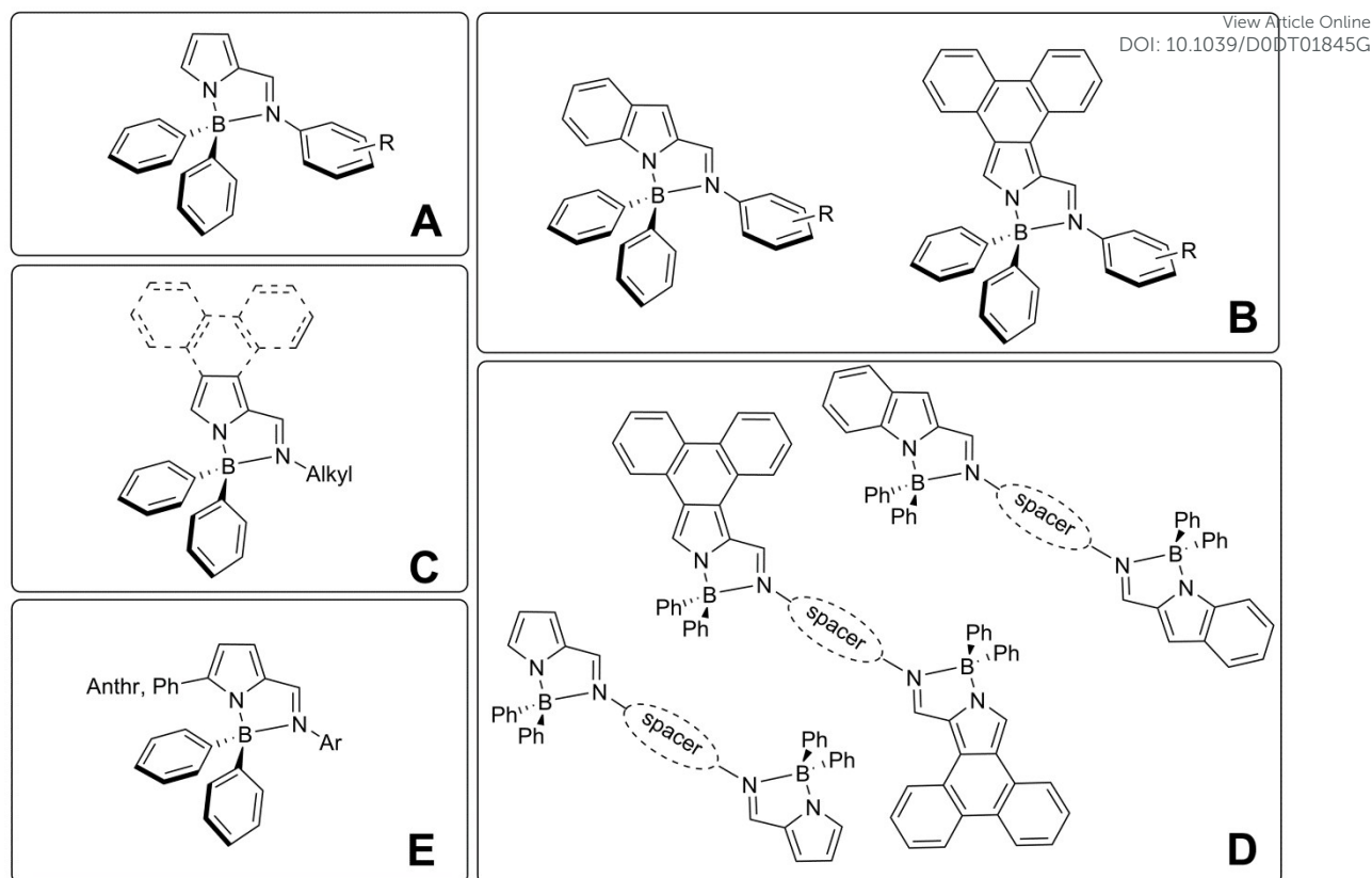
Chart 1. 2-( N -arylformimino)pyrrolyl-BPh 2 complexes previously reported by our research group.
