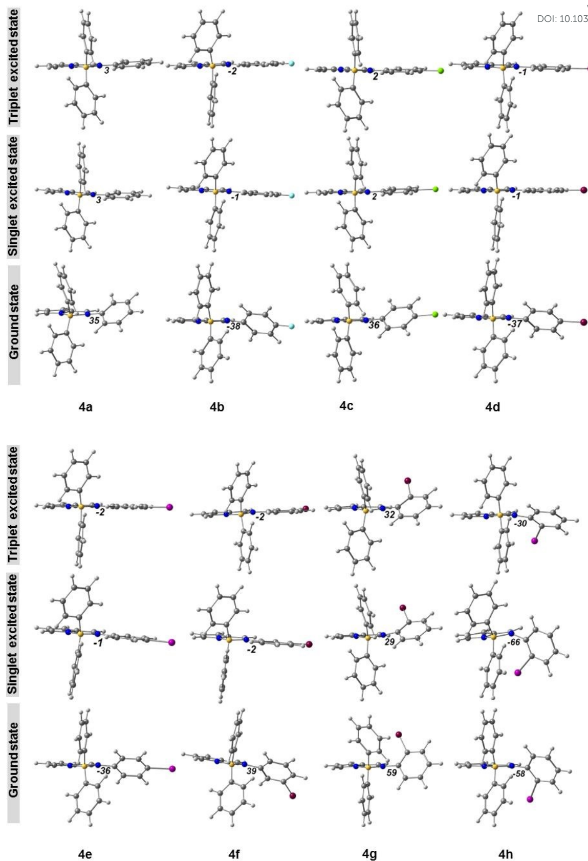
Figure 4. Calculated geometries of the ground state (DFT) and of the first singlet and triplet excited states (TDDFT) of the complexes 4a-4h ; the numbers represent the C6-N2-C7-C8 dihedral angle (°) for each species.
