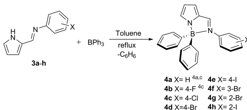
Scheme 2. Synthesis of the 2-( N -arylformimino)pyrrolyl-BPh 2 complexes 4a-4h .
