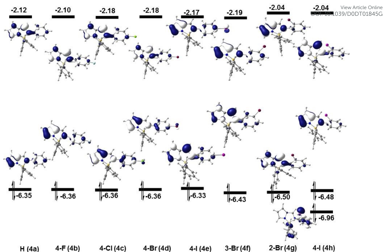
Figure 5. Energies of the HOMOs and LUMOs of complexes 4a-4h and HOMO-1 of 4h with their 3D representation (arrows indicate double occupation of the HOMOs).
