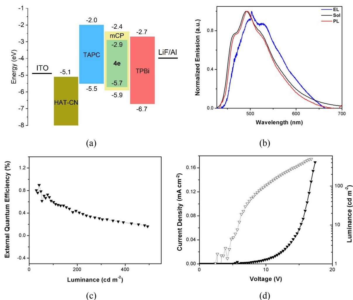
Figure 7. Characteristics of OLED devices fabricated using complex 4e as the emitter and mCP as host: (a) Schematic device energy level structure; (b) Electroluminescence spectra (EL) compared with the film photoluminescence (PL) and solution fluorescence spectra in THF (Sol); (c) External Quantum Efficiency (EQE) vs. Luminance; and (d) Current Density (filled symbols)/Luminance (open symbols) vs. Voltage.
