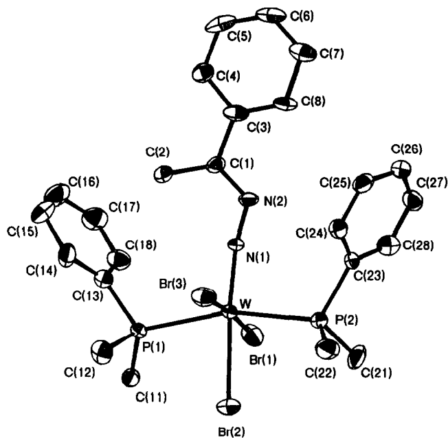
Fig. 1. ORTEP drawing of 6d .
