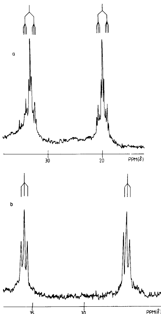
Fig. 2. ^{31}P\{^1H\} NMR spectra of Mo_3S_4Br_4 \cdot 3dpppe (a) and Mo_3S_4Cl_4 \cdot 3dpppe (b) in CH_2Cl_2/C_6D_6 at 25 °C.
