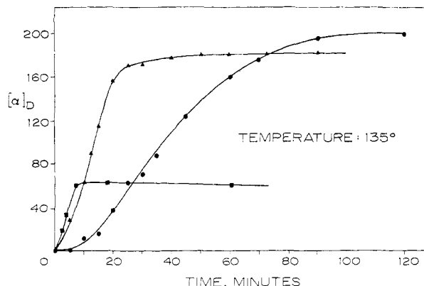
Figure 1. Development of optical activity in samples of neat, crystalline 1,1'-binaphthyl at 135^\circ : ●, samples as crystallized from acetone; 8 ▲, same material ground into smaller crystals; ■, more finely ground samples. [\alpha]_D is the specific rotation of an individual sample dissolved in benzene for analysis of optical activity.
