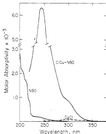
Figure 1. Spectral evidence for \pi -complex formation (spectra taken in ethanol).
