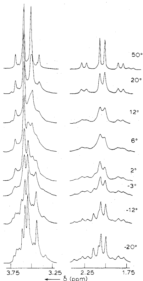
Figure 2. Temperature-variation profile of the proton NMR signals of cis -[Pt(DMSO)(C 3 H 6 )Cl 2 ] in CDCl 3 . The downfield sets of resonances correspond to the DMSO protons; those to higher fields refer to the olefinic methyl protons.
