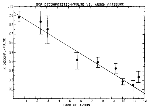
Figure 4. Fraction of bicyclopropyl decomposed per pulse vs. pressure of Ar bath gas (6.1 J/cm 2 ).
