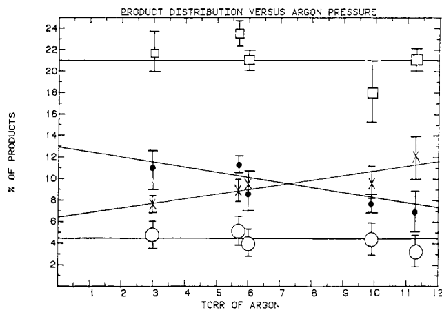
Figure 5. Partial product distribution vs. pressure of Ar bath gas: (□) butadiene, (●) 3-methylcyclopentene, (×) allylcyclopropane, (○) 1-butene (6.1 J/cm 2 ).
