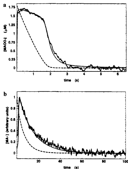
Figure 2. (a) Solid line: experimental data of the peroxymalonyl radical kinetics. Conditions: 7 \times 10^{-3} M Ce(IV), 0.5 M MA, 1 M \text{H}_2\text{SO}_4 . EPR settings: microwave power 110 mW, modulation amplitude 8 G. Dotted line: calculated kinetics of the peroxymalonyl radical. Dashed line: calculated decay of the oxygen concentration. (b) Solid line: experimental data of the malonyl radical kinetics. Chemical conditions: same as in part a. EPR settings: microwave power 11 mW, modulation amplitude 4 G. Dotted line: calculated kinetics of the malonyl radical. Dashed line: calculated kinetics of the Ce(IV) decay.
