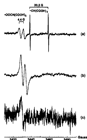
Figure 1. EPR spectrum observed from the reaction of Ce(IV) with MA under oxygen atmosphere. Chemical conditions: 3.3 \times 10^{-3} M Ce(IV), 0.5 M MA, 1 M \text{H}_2\text{SO}_4 . EPR settings: (a) microwave power 11 mW, modulation amplitude 2 G, and (b) microwave power 110 mW, modulation amplitude 8 G. (c) EPR spectrum of deuterio-peroxymalonyl radical obtained under the same conditions as spectrum a.
