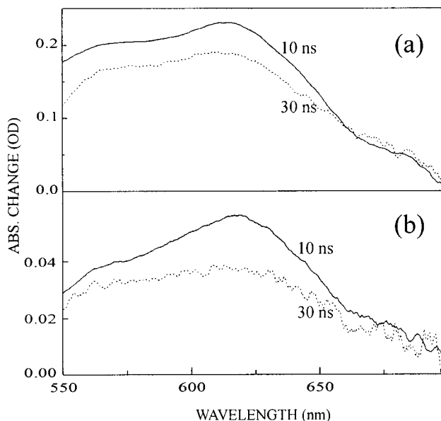
Figure 8. Transient-absorption spectra of MVCl 2 ( 1 \times 10^{-3} M) ethanol solutions with I (a) and II (b) at two given delay times after 266-nm excitation.
