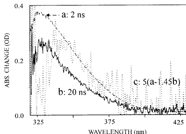
Figure 6. Transient-absorption spectra of II in cyclohexane at 2- (a) and 20-ns (b) delay times after 266-nm excitation and a difference spectrum (c) simulated from 5 (a - 1.45b).
