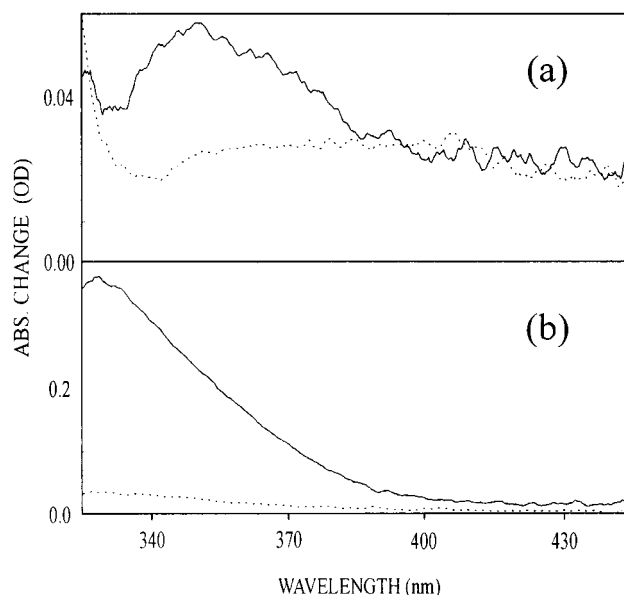
Figure 7. Transient-absorption spectra, at 10-ns delay after 266-nm excitation, of I (a) and II (b) in cyclohexane (solid) and in the 19:1 (v:v) mixture of cyclohexane and MVCl 2 -saturated ethanol (dotted).
