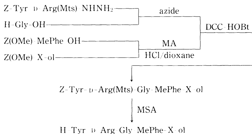
Fig. 3. Synthetic Scheme for H-Tyr-D-Arg-Gly-MePhe-X-ol (X=Leu or Ile)
