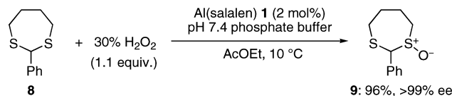
Scheme 12. Oxidation of an Acyclic Dithioacetal 10
