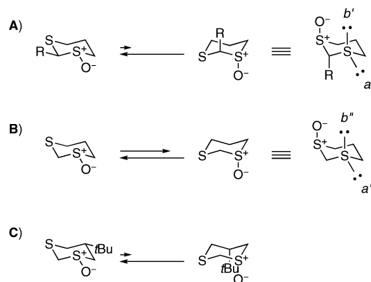
Scheme 5. Conformational Issue of 2-Substituted 1,3-Dithiane 1-Oxide (A), 1,3-Dithiane 1-Oxide (B), and 5- tert -Butyl-1,3-dithiane 1-Oxide (C)
