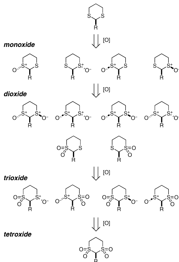
Scheme 1. Product Complexity in Oxidation of 2-Substituted 1,3-Dithianes
