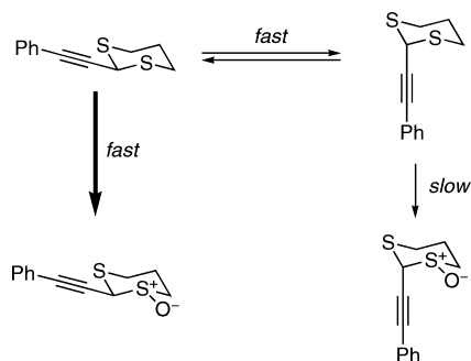
Scheme 10. Asymmetric Oxidation of 1,3-Dithiolanes 5
