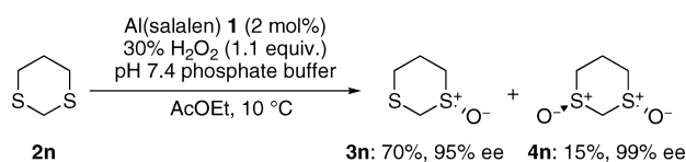
Scheme 4. Asymmetric Synthesis of trans -1,3-Dithiane 1,3-Dioxide 4n
