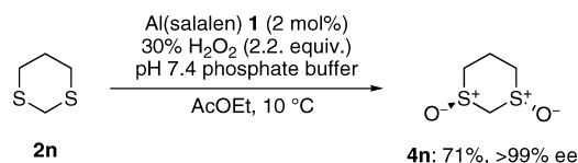
Scheme 4. Asymmetric Synthesis of trans -1,3-Dithiane 1,3-Dioxide 4n
