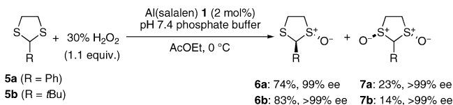
Scheme 10. Asymmetric Oxidation of 1,3-Dithiolanes 5
