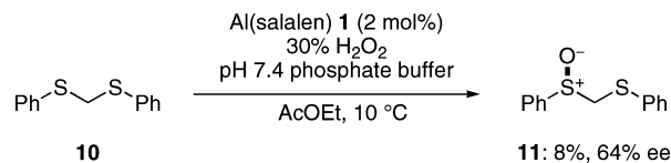
Scheme 12. Oxidation of an Acyclic Dithioacetal 10
