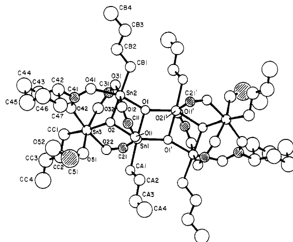
Figure 4. ORTEP plot of [(n\text{-BuSn}(\text{O})\text{O}_2\text{CC}_6\text{H}_{11})_2(n\text{-BuSn}(\text{O}_2\text{CC}_6\text{H}_{11})_3)_2] (3) from isotropic refinement of 49 of the 62 independent non-hydrogen atoms. Carbon atoms of only two of the cyclohexyl groups are shown. The 10 carboxylate carbon atoms are shaded. Primed atoms are related to unprimed ones by the inversion operation.
