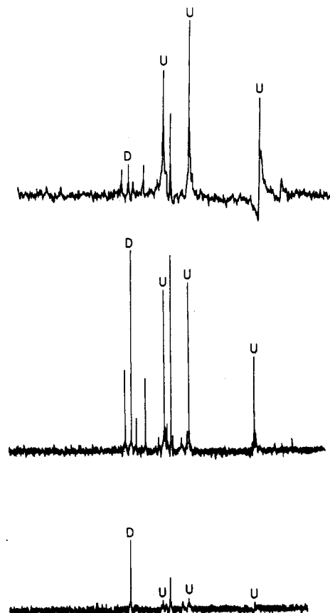
Figure 6. ^{119}\text{Sn} NMR spectra of [(n\text{-BuSn}(\text{O})\text{O}_2\text{CC}_6\text{H}_{11})_2(n\text{-BuSn}(\text{O}_2\text{CC}_6\text{H}_{11})_3)]_2 (3) in \text{CDCl}_3 , indicating hydrolysis to a "drum" form. The frequencies, which are listed in Table V, remain the same from spectrum to spectrum. The upper spectrum is for a sample containing \text{P}_4\text{O}_{10} , added to reduce hydrolysis relative to the sample used for the middle spectrum, which has no added drying agent. The lower spectrum was recorded on the latter sample 1 week later. D identifies the line due to the drum formulation and U, the lines due to the unfolded drum. The remainder are lines due to intermediates.
