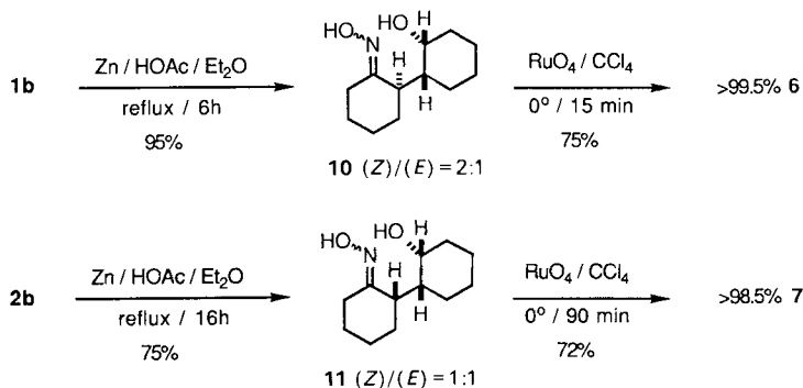
Scheme 6
