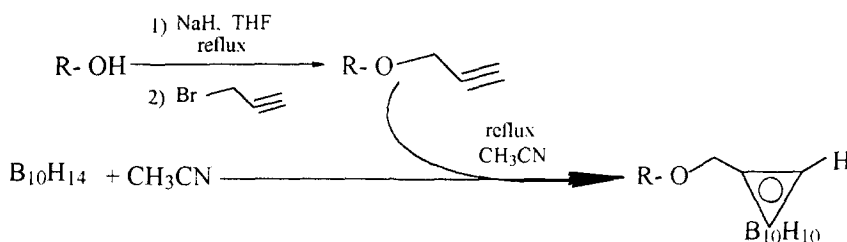
Scheme 2: Heying's general method.
