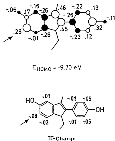
Fig. 1. HOMO and \pi -charge of 3a on the basis of \pi -VSCF calculations [11]; a fully geometry optimized coplanar structure was calculated throughout
