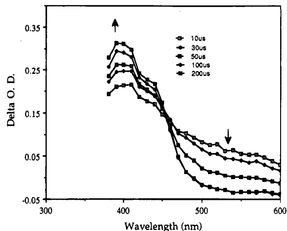
Figure 5. Transient absorption spectra obtained from laser flash photolysis of 1e in \text{CH}_2\text{Cl}_2 containing 0.35 M triphenylmethane. Spectra were taken 10–200 \mu\text{s} after the laser pulse.
