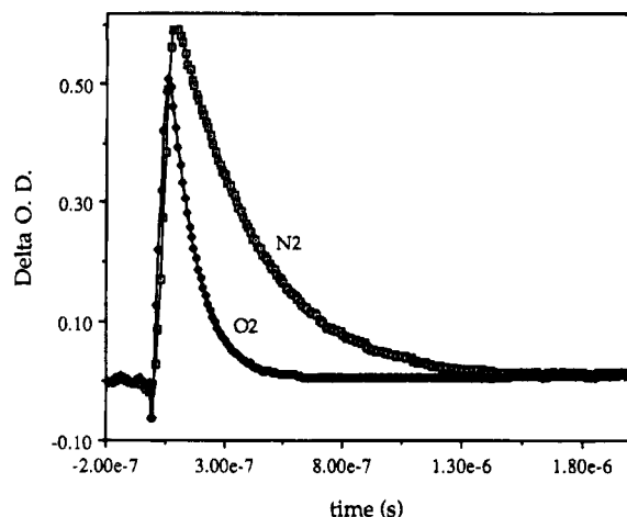
Figure 4. Transient absorption waveforms at 400 nm obtained from laser flash photolysis of 1e in \text{N}_2 -purged and \text{O}_2 -purged \text{CH}_3\text{CN} .
