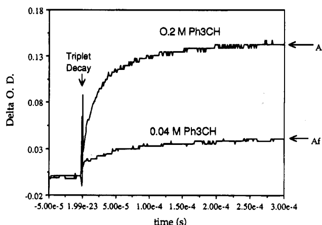
Figure 6. Transient absorption waveforms at 370 nm obtained from laser flash photolysis of 1e in \text{CH}_2\text{Cl}_2 containing 0.040 and 0.20 M triphenylmethane. The feature near 0 \mu\text{s} is the growth and decay of the excited triplet state of 1e (Figure 3).
