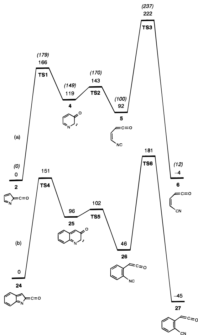
Figure 9. Schematic potential profiles showing retro-Wolff rearrangements of (a) 2-carbonyl-2H-pyrrole ( 2 ) and (b) 2-carbonyl-2H-indole ( 24 ) (B-LYP/6-311+G(2d,p)+ZPVE, with G2(MP2,SVP) values in italics, kJ mol -1 ).
