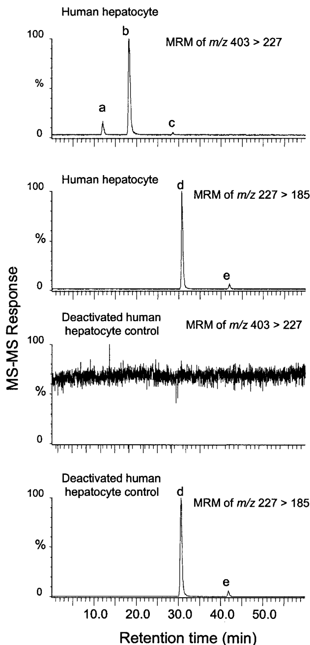
Fig. 3. Negative ion electrospray multiple reaction monitoring LC-UV-MS-MS analysis of resveratrol incubated for 4 h with human hepatocytes or deactivated human hepatocytes (control). Peaks were assigned to the following compounds. (a) trans -resveratrol-4'- O -glucuronide; (b) trans -resveratrol-3- O -glucuronide; (c) cis -resveratrol-3- O -glucuronide; (d) trans -resveratrol; (e) cis -resveratrol.
