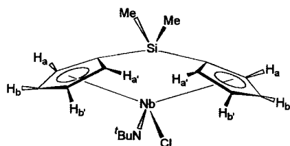
Figure 1. Proposed structure for [\text{Me}_2\text{Si}(\eta^5\text{-C}_5\text{H}_4)_2]\text{Nb}(=\text{N}'\text{Bu})\text{Cl} ( 1 ).
