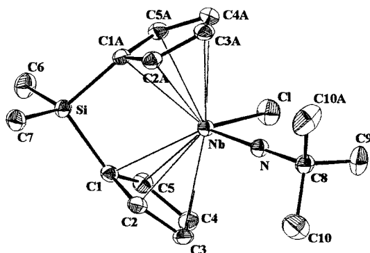
Figure 2. Molecular structure and atom-labeling scheme for [\text{Me}_2\text{Si}(\eta^5\text{-C}_5\text{H}_4)_2]\text{Nb}(=\text{N}'\text{Bu})\text{Cl} ( 1 ).
