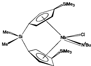
Figure 5. Proposed structure for meso -[Me 2 Si(η 5 -C 5 H 3 -SiMe 3 ) 2 ]Nb(=N'Bu)Cl ( 6 ).
