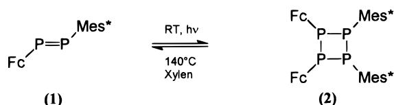
Scheme 1 a
