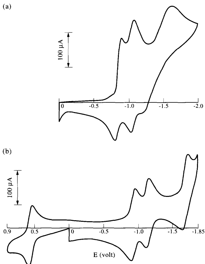
Fig. 3. Cyclic voltammograms of \text{HL-NO}_2 (a) and its complexes 1 (b) in \text{CH}_3\text{CN} with a glassy carbon electrode at a scan rate of 100 \text{ mVs}^{-1} .
