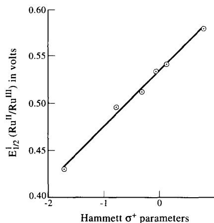
Fig. 2. Plot of E_{1/2}^I (Ru II /Ru III couple) vs the Hammett \sigma^+ parameters with a linear least-squares fit to the data.
