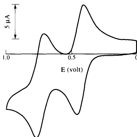
Fig. 1. Cyclic voltammogram of 6 in CH 3 CN with a platinum electrode at a scan rate of 100 mVs −1 .
