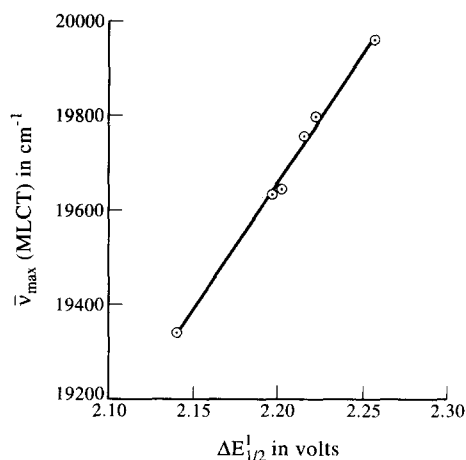
Fig. 4. Correlations between the redox potential, \Delta E_{1/2}^I and the energy of the MLCT band maxima for the complexes listed in Table 1.
