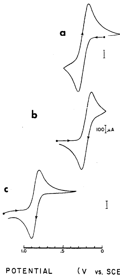
Fig. 4. (a) Reversible oxidation of \text{Mn}(\text{NCMe}) in acetonitrile containing 0.1 M TEAP at -35^\circ\text{C} and a scan rate of 50 \text{ mV s}^{-1} . (b) Reversible reduction of the solution in (a) after exhaustive oxidation of 0.5 V and -35^\circ\text{C} . (c) Cyclic voltammogram (initial negative scan) of the solution in (b) immediately after the addition of excess \text{P}(\text{OPh})_3 .
