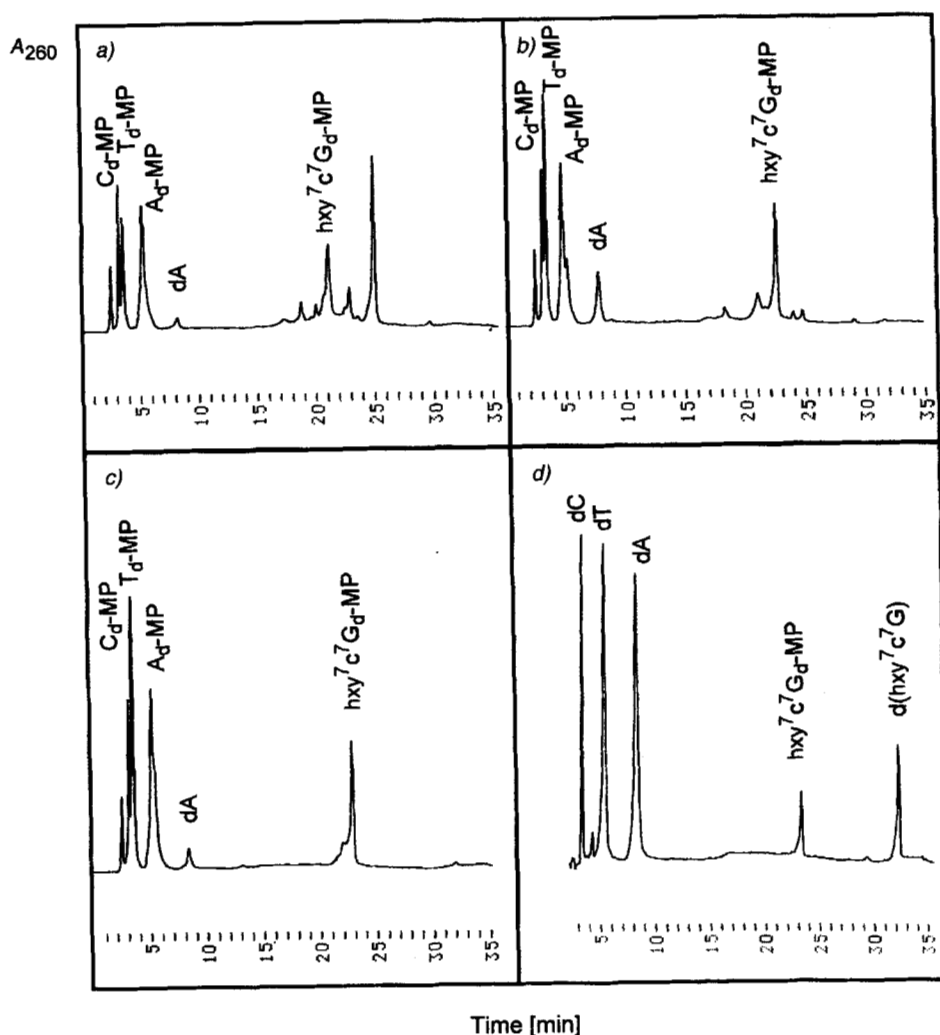
Fig. 4. Reversed-phase HPLC pattern (RP-18) of the reaction products obtained during enzymatic hydrolysis of oligonucleotide 23 by snake-venom phosphodiesterase at 37° after a) 10 min, b) 1 h, c) 30 h, and d) 30 h after subsequent addition of alkaline phosphatase. For details, see Exper. Part .
