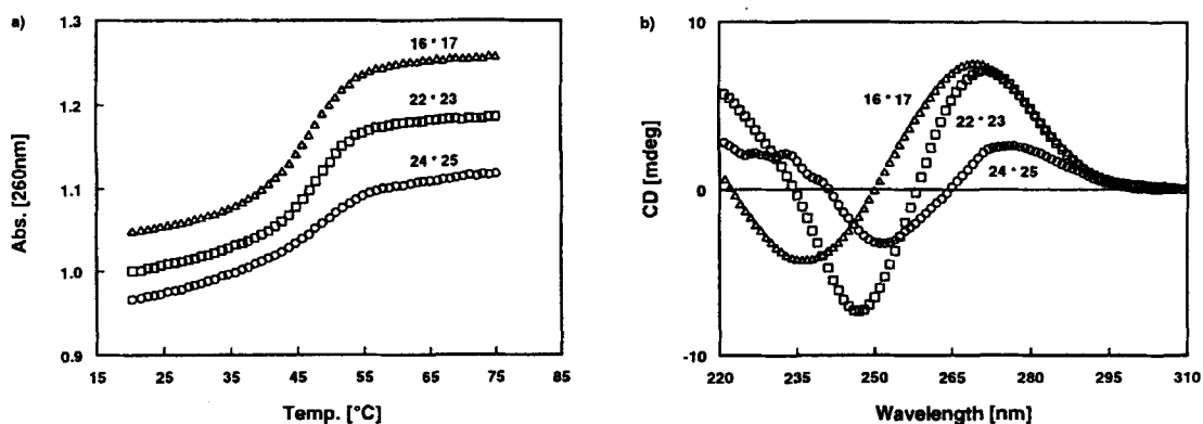
Fig. 2. a) Melting profiles of hybrids 16 · 17 , 22 · 23 , and 24 · 25 (see Table 4) measured at 260 nm (oligomer concentration, 10 \mu M of single strands; conditions, see Fig. 1, a) and b) CD spectra of hybrids 16 · 17 , 22 · 23 , and 24 · 25 measured at 20° at 10 \mu M single-strand concentration (conditions, see Fig. 1, a)
