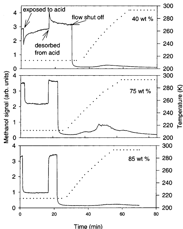
Figure 1. Uptake and desorption of methanol at 213.1 K, followed by heating to room temperature, for 40, 75, and 85 wt % \text{H}_2\text{SO}_4 (chosen as most representative data). Heating curves for each experiment are indicated by the dotted lines, scaled to the right axis. The 40 wt % \text{H}_2\text{SO}_4 shows significant low-temperature methanol desorption, only trace amounts of methanol desorbed at 75 wt %, and no desorption occurred at 85 wt % \text{H}_2\text{SO}_4 at 213.1 K. Once the methanol flow was shut off and the baseline level was achieved, the samples were heated to room temperature.
