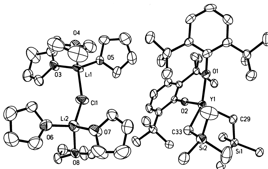
Fig. 1. Thermal ellipsoid plot of \{(\text{Me}_3\text{SiCH}_2)_2\text{Y}(\text{OC}_6\text{H}_3^t\text{Bu}_2-2,6)_2\} \{[(\text{THF})_3\text{Li}]_2\text{Cl}\} , 2 , drawn at the 50% probability level.
