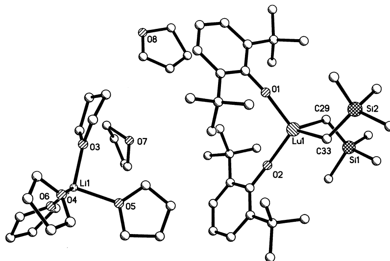
Fig. 2. Ball and stick plot of \{(\text{Me}_3\text{SiCH}_2)_2\text{Lu}(\text{OC}_6\text{H}_3^t\text{Bu}_2\text{-2,6})_2\}[\text{Li}(\text{THF})_4](\text{THF})_2 , 3 .
