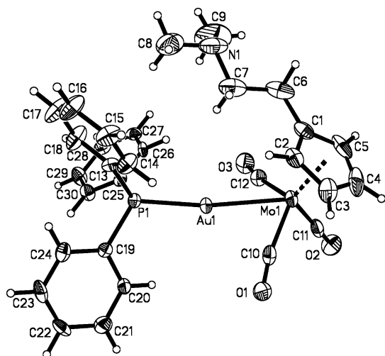
Figure 8. Molecular structure of 8 (50% thermal ellipsoids). Selected bond lengths (Å) and angles (deg): Au–Mo = 2.7208(6), Au–C(10) = 2.547(6), Au–C(12) = 2.524(6), Mo–C(1) = 2.345(6), Mo–C(2) = 2.362(6), Mo–C(3) = 2.351(6), Mo–C(4) = 2.308(7), Mo–C(5) = 2.302(6), Mo–C(10) = 1.947(6), Mo–C(11) = 1.946(7), Mo–C(12) = 1.947(7), O(1)–C(10) = 1.176(6), O(2)–C(11) = 1.171(7), O(3)–C(12) = 1.153(7), P–Au–Mo = 171.25(4), C(10)–Mo–C(12) = 107.4(3), C(10)–Mo–C(11) = 83.1(3), C(11)–Mo–C(12) = 81.5(3), C(11)–Mo–Au = 117.45(19), C(10)–Mo–Au = 63.62(17), C(12)–Mo–Au = 62.93(18), O(1)–C(10)–Mo = 169.4(5), O(2)–C(11)–Mo = 179.0(6), O(3)–C(12)–Mo = 170.3(6).
