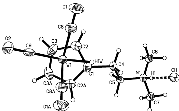
Figure 4. Molecular structure of 4 (50% thermal ellipsoids). Selected bond lengths (Å) and angles (deg): W–H(1W) = 1.75(9), W–C(1) = 2.373(9), W–C(2) = 2.345(6), W–C(2A) = 2.346(6), W–C(3/3A) = 2.306(7), W–C(8/8A) = 1.971(7), W–C(9) = 1.969(10), C(8/8A)–O(1/1A) = 1.147(8), C(9)–O(2) = 1.173(12), N···Cl = 3.066(7), C(8A)–W–C(8) = 106.5(4), C(9)–W–C(8/8A) = 80.6(3), O(1/1A)–C(8/8A)–W = 178.3(7), O(2)–C(9)–W = 178.0(10).
