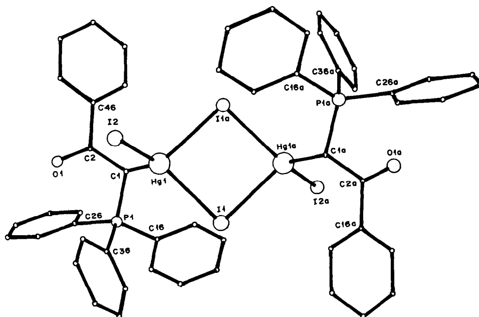
Fig. 2. Molecular structure and atom numbering scheme for [(C_6H_5)_3PCHCOC_6H_5 \cdot HgI_2]_2 .
