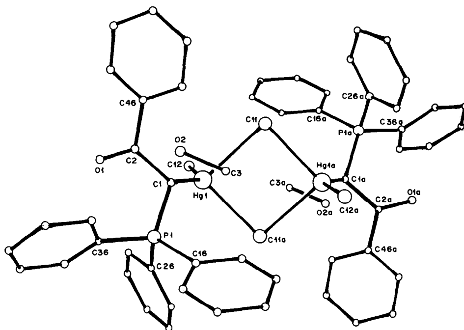
Fig. 1. Molecular structure and atom numbering scheme for [(C_6H_5)_3PCHCOC_6H_5 \cdot HgCl_2]_2 \cdot 2CH_3OH .
