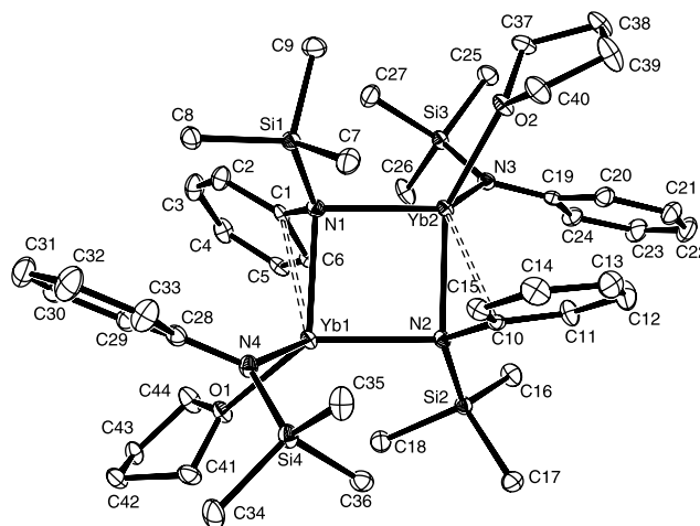
Fig. 1. Molecular structure and atom numbering scheme for [Yb{NPh(SiMe 3 ) 2 }(THF)] 2 ( 2a ).
