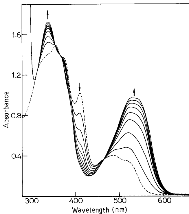
Fig. 4. Spectra of pure \text{L}^1\text{Pd}_2\text{Cl}_2 (---) and a reaction mixture of \text{L}^1\text{Pd}_2\text{Cl}_2 and m\text{-CPBA} (—) at 300 K in \text{CHCl}_3 solution. The arrows indicate increase and decrease of band intensities as the reaction proceeds.
