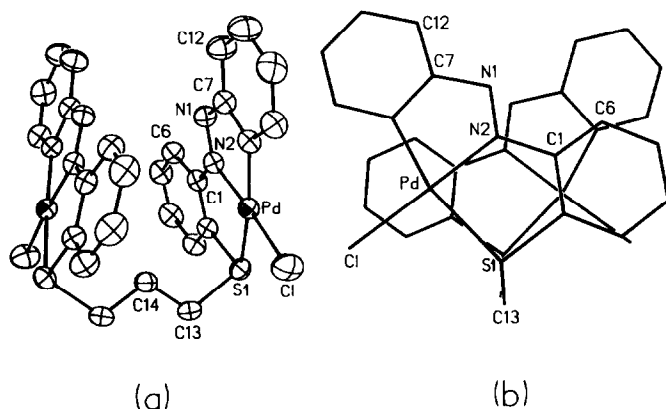
Fig. 1. (a) ORTEP diagram and atom labelling of L^1Pd_2Cl_2 . All atoms are represented by their 40% probability ellipsoids. (b) Molecular view of L^1Pd_2Cl_2 projected approximately along the S \cdots S axis.
