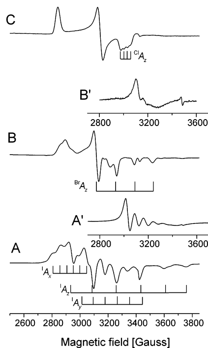
Figure 10. EPR spectra of oxidized complex 7 with various apical ligands in toluene/dichloromethane solution (30/70 v/v): A, 7-I , 77 K; A', 298 K; B, 7-Br , 77 K; B', 298 K; C, 7-Cl , 77 K. The resolved hyperfine splittings due to 127 I, 79,81 Br, or 35,37 Cl in anisotropic spectra are marked. Conditions: microwave frequency, \nu = 9.573 GHz for anisotropic spectra and 9.782 GHz for isotropic spectra; microwave power, 12.5 mW; modulation amplitude, 8 G; modulation frequency, 100 kHz.
