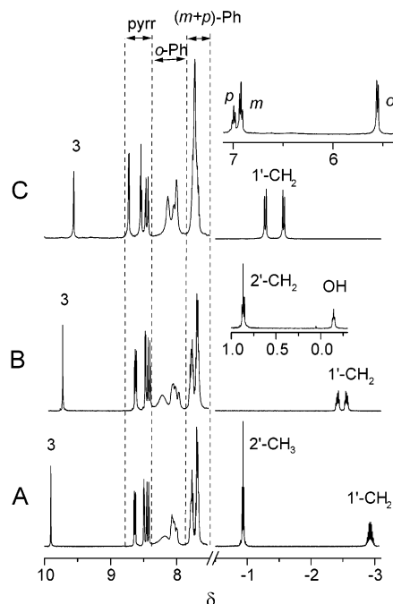
Figure 1. ^1\text{H} NMR spectra (500 MHz, \text{CDCl}_3 , 298 K) of 21-alkylated nickel(II) complexes of an inverted porphyrin: A, 3 ; B, 4 ; C, 7 . Assignments: pyr, \beta -pyrrole; 3, inverted pyrrole; o -, m -, p -Ph, ortho , meta , para protons of meso -phenyls; o , m , p , ortho , meta , para protons of benzyl substituent in 7 ; 1', methylene group attached directly to 21-C.
