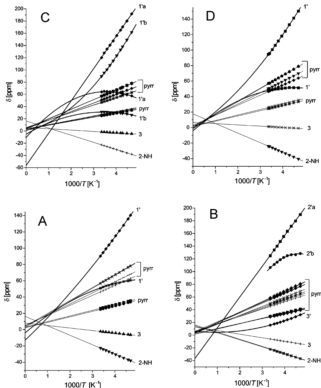
Figure 5. Curie plots of 4 -HCl (A), 5 -HCl (B), 6 -HCl (C), and 7 -HCl (D) based on the data taken for \text{CDCl}_3 solutions of respective systems. The assignments “a” and “b” are introduced to distinguish the diastereomers but are not related to labeling of the diamagnetic precursors in Figure 3. The nonlinear dependencies have been traced by means of a second-order polynomial fitting procedure but are drawn only to join the experimental points.
