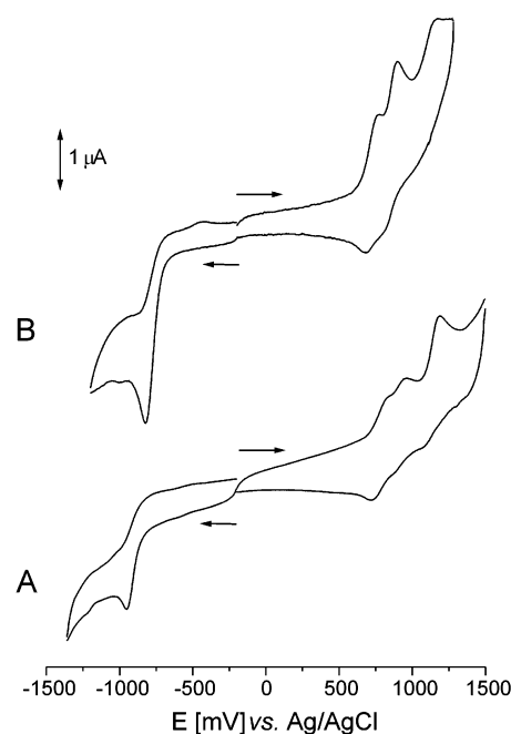
Figure 9. Cyclic voltammograms of 10 (A) and 11 (B) in CH 2 Cl 2 solutions (supporting electrolyte, 0.1 M TBAP; working electrode, glassy carbon disk; reference electrode, Ag/AgCl; auxiliary electrode, platinum wire; scan rate, 50 mV s −1 ).
